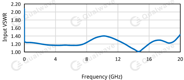
Input VSWR (J0) vs. Frequency
