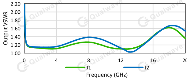
Output VSWR (Off state) vs. Frequency
