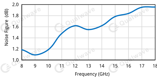
Noise Figure vs. Frequency
