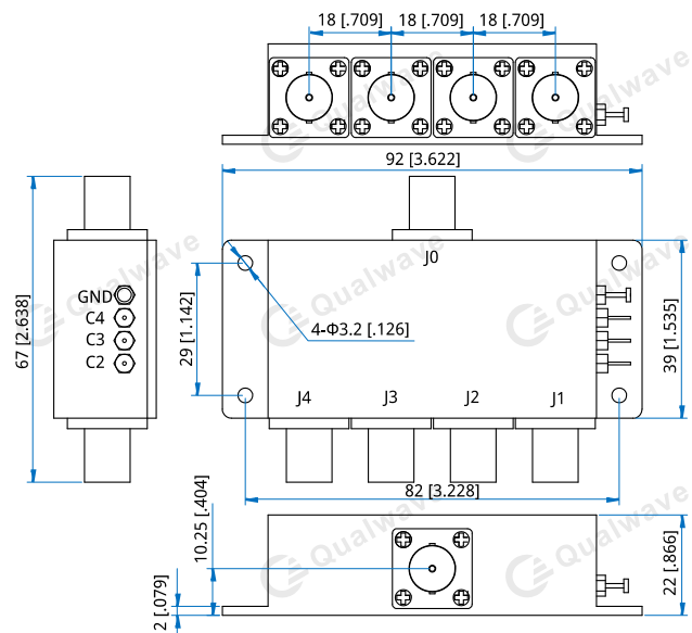
Outline B
