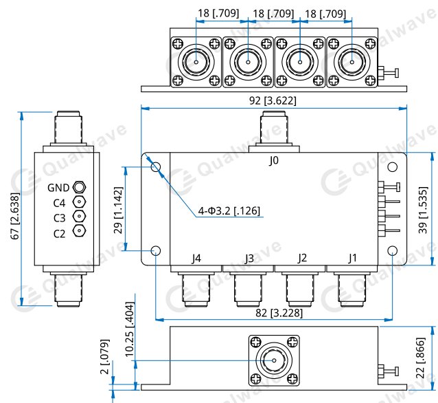
Outline A
