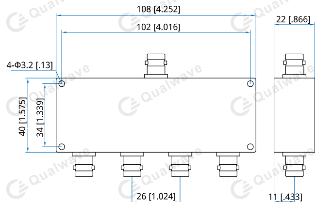
Outline B
