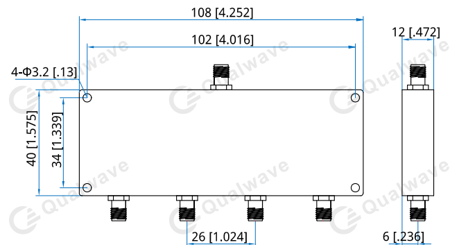
Outline A
