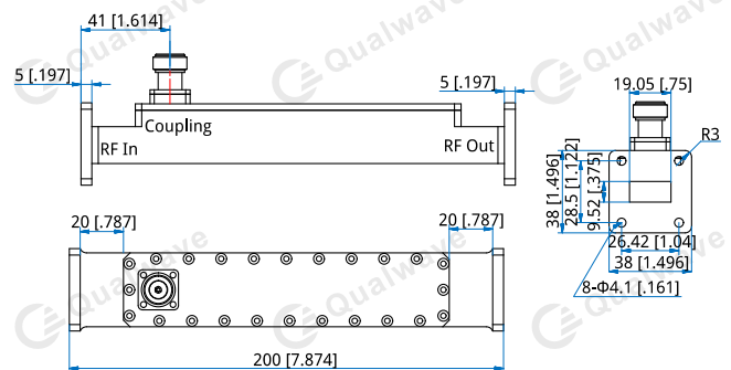
Outline B
